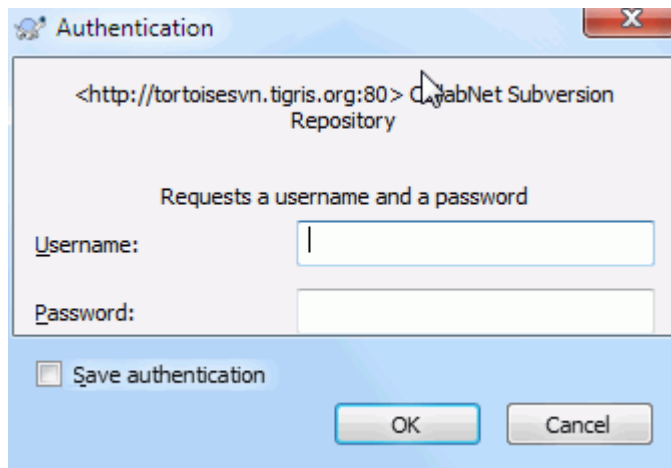
Figure 4.5. Authentication Dialog
