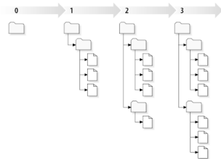
Figure 2.7. The Repository
